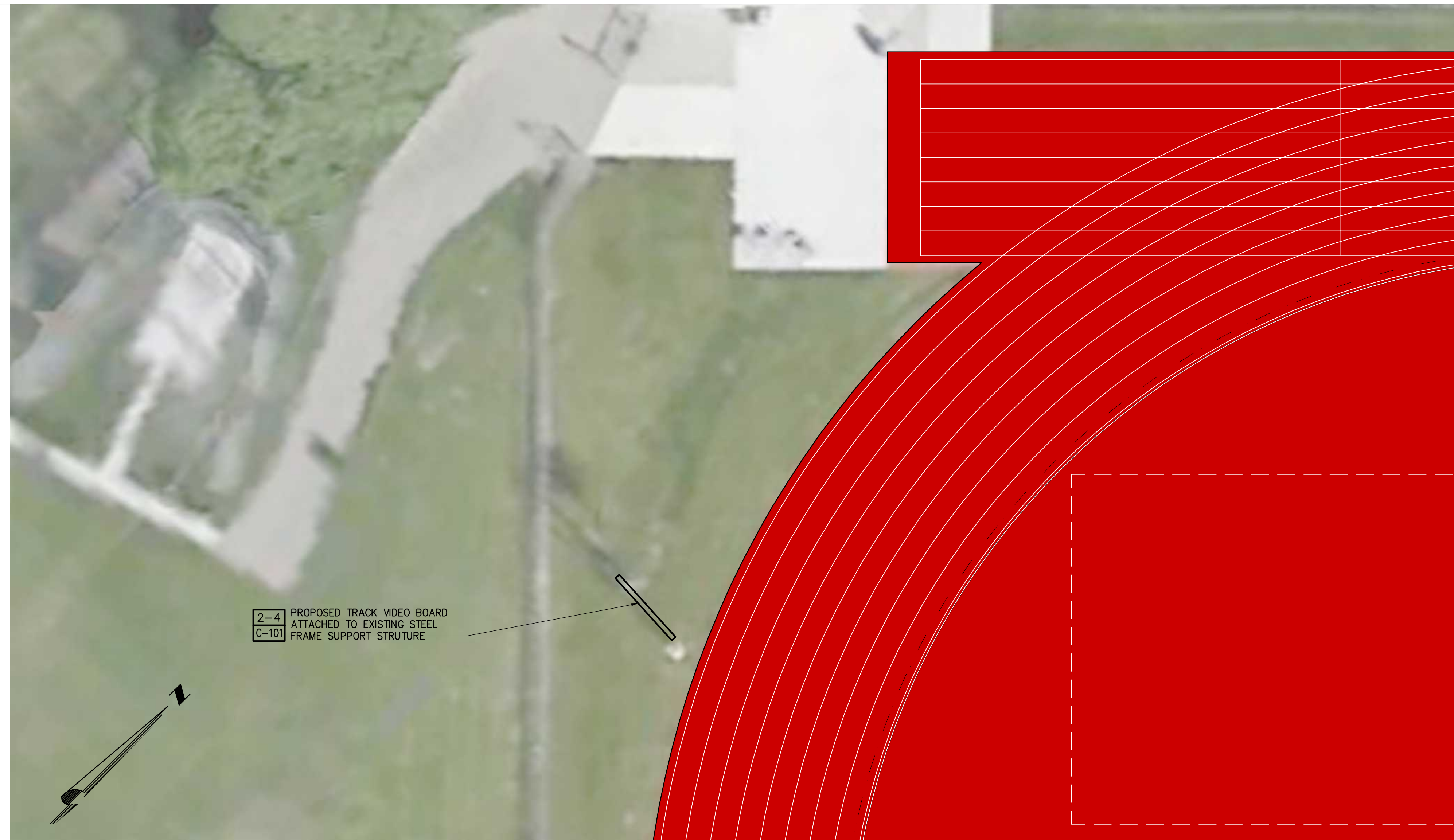
1 ENLARGED LAYOUT PLAN SCALE: 1"=10'
