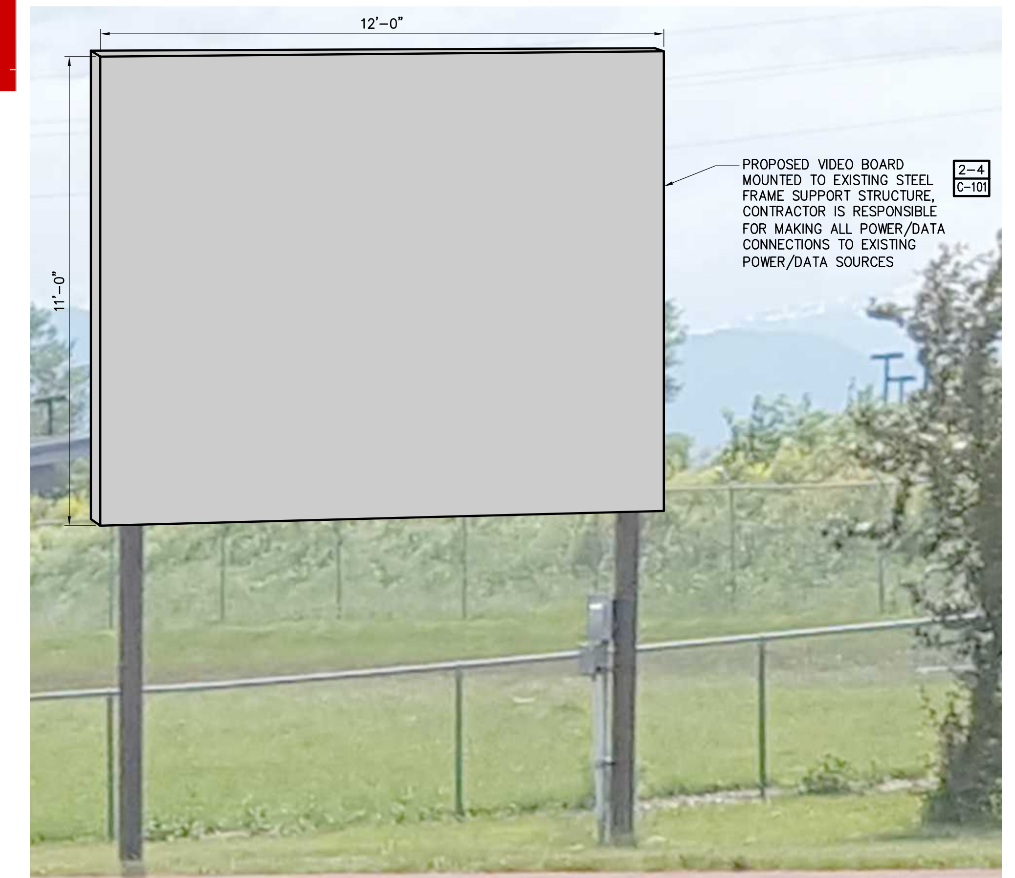
4 PROPOSED VIDEO BOARD MOUNTING SCALE:
